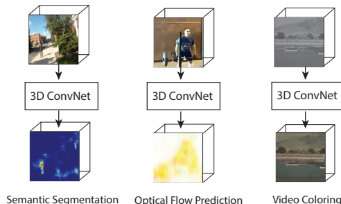
Figure 1. Voxel to voxel prediction: is a fine-grained video understanding task where the algorithm need to infer a variable for each input voxel. The problem has many potential applications including video semantic segmentation, optical flow prediction, depth estimation, and video coloring.
